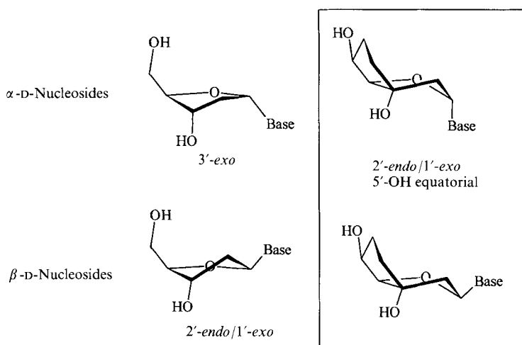
Fig. 3. Preferred conformations of \alpha -D- and \beta -D-deoxyribonucleosides, and of \alpha -D- and \beta -D-bicyclobutynucleosides
