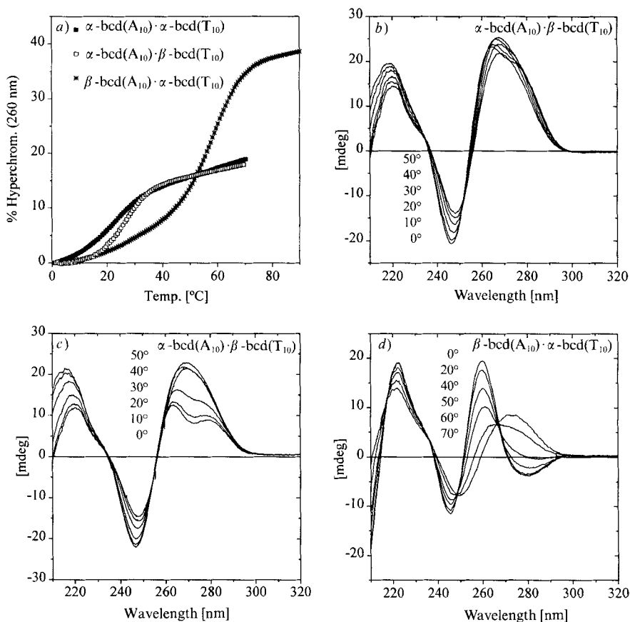
Fig. 10. a) UV/Melting curves and b) c) d) CD spectra of the bicyclo-DNA duplexes indicated (10 mM NaH 2 PO 4 , 1M NaCl, pH 7.0, c = 5.2 – 6.7 \mu\text{M} )
