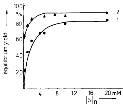
Fig. 5. The equilibrium yield of 1 and 2 as a function of reactant starting concentration [S]_0 (C/N-ratio 1 : 1) in ethyl acetate/phosphate buffer (1 M , pH 7), \alpha = 25 , total volume 52 ml, \alpha -chymotrypsin 20 mg/ml buffer
