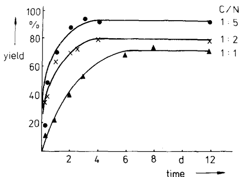
Fig. 4. Kinetics of the synthesis of 1 at different nucleophile content in ethyl acetate/phosphate buffer (1 M, pH 7), \alpha = 50 , total volume 51 ml, [Z-Tyr-OH] = 5 mM, 20 mg \alpha -chymotrypsin
