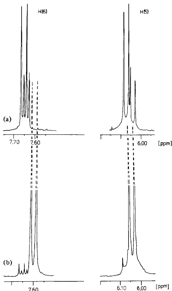
Fig. 1. 300 MHz 1 H NMR spectra (lowfield region only, D 2 O, pD 5, 0.02 mmol/l) of trans -[(NH 3 ) 2 Pt(mec) 2 ] 2+ (a) and trans -[(NH 3 ) 2 Pt(mec)Cl]Cl after 4 weeks at 40 °C (b). Resonances due to trans -[(NH 3 ) 2 Pt(mec) 2 ] 2+ formed appear after only a few days.
