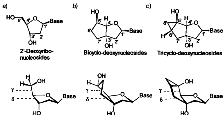
Fig. 1. a) 2'-Deoxyribonucleosides containing the nucleobases adenine, thymine, guanine, and cytosine. b) Bicyclo-deoxynucleosides [6]. c) Tricyclo-deoxynucleosides (= 2'-deoxy-3'5'-ethano-5',6'-methano- \beta -D-ribonucleosides (or 2'-deoxy-3',5',5'-propane[1,2,3]triyl- \beta -D-ribonucleosides), see Footnote 2) of the natural nucleobase thymine and the N^6 -benzoyl-protected adenine
