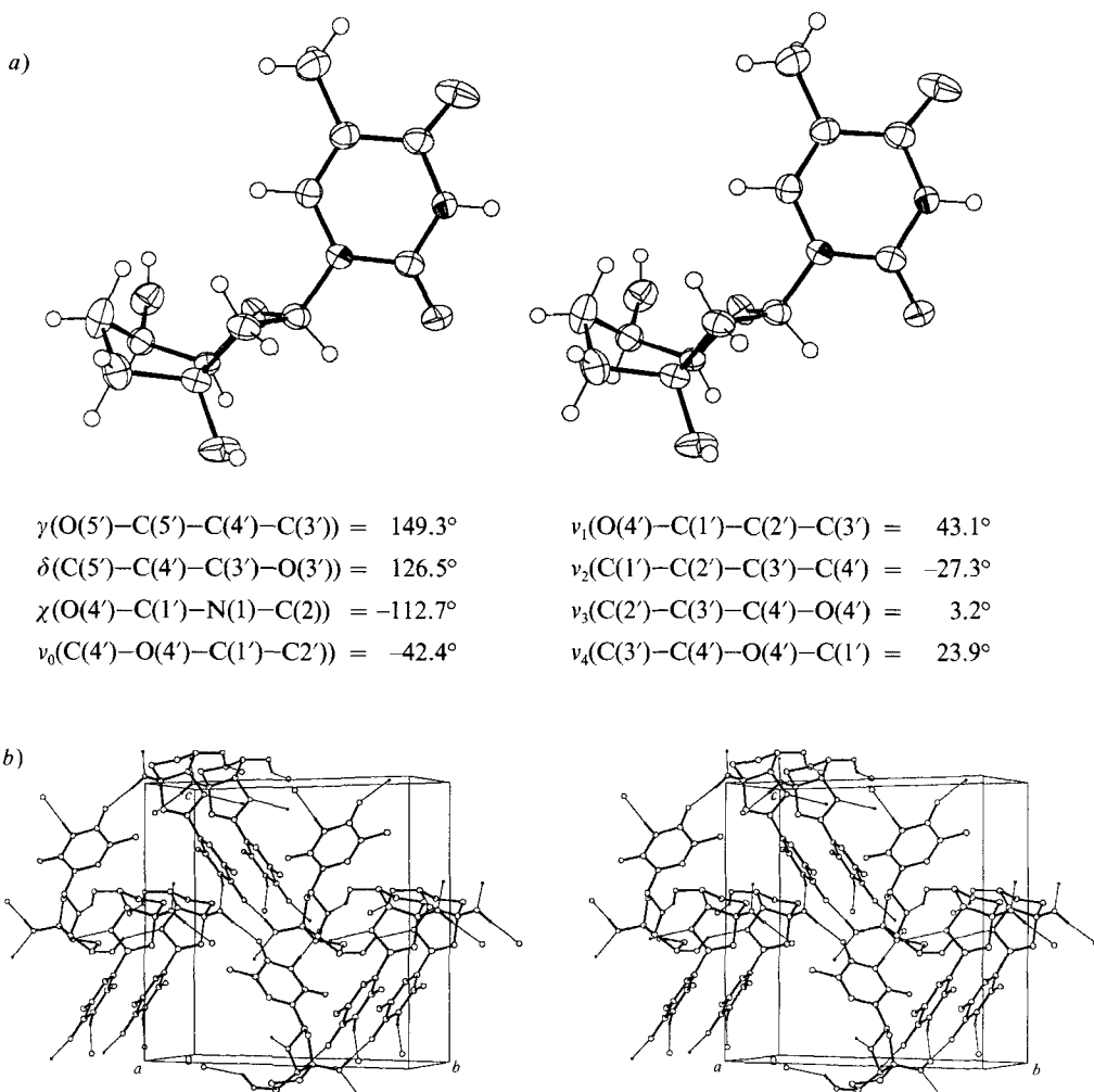
Fig. 5. X-Ray structure of bicyclothymidine 1 : a) ORTEP plot (stereoscopic view, 50%-probability thermal ellipsoids) including selected torsion angles and b) stereoscopic view of the asymmetric unit
