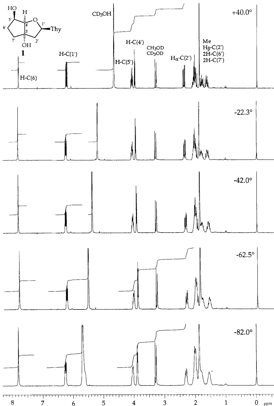
Fig. 6. ^1\text{H-NMR} spectra (400 MHz, \text{CD}_3\text{OD} ) of bicyclothyminidine 1 at temperatures between +40 and -82°
