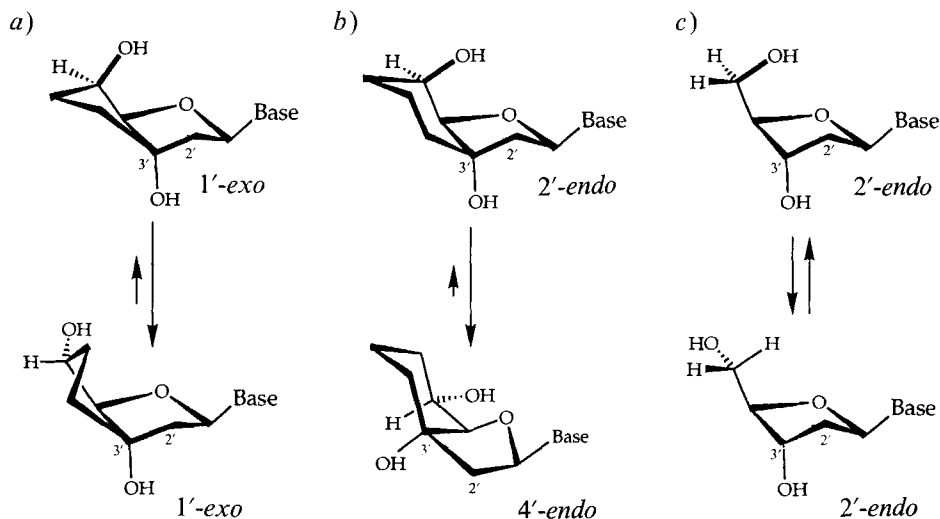
Fig. 9. Conformational drawings of nucleosides with torsion angle \gamma corresponding to a + sc - (upper) and ap -conformation (lower): a) bicyclonucleosides with a five-membered carbocyclic ring (this communication), b) bicyclonucleosides with a six-membered carbocyclic ring, and c) natural 2'-deoxyribonucleosides
