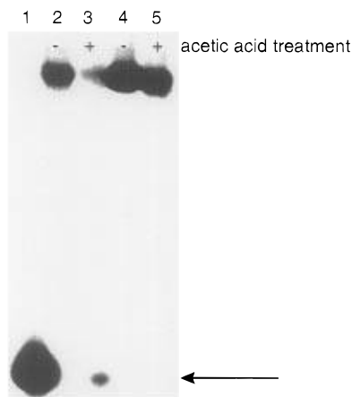
Figure 8. Autoradiogram of 20% denaturing polyacrylamide gel demonstrating the topoisomerase I-mediated formation of the phosphoramidate linkage. Lane 1, synthetic 13-mer cleavage product 5' 32 pGGCGCGGAGACTT; lane 2, ligation product derived from IV ; lane 3, ligation product derived from IV + acetic acid; lane 4, ligation product derived from I ; lane 5, ligation product derived from I + acetic acid.
