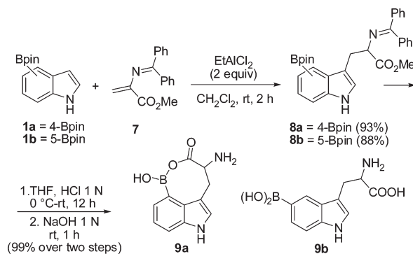
Scheme 4. Friedel–Crafts Alkylation of Boronated Indoles 1a,b with Methyl 2-(Diphenylmethyleamino)acrylates 7 and Hydrolysis of Compounds 8a,b
