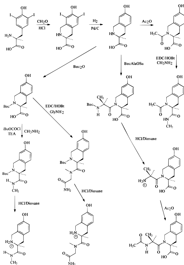
Figure 1. Synthetic scheme.
