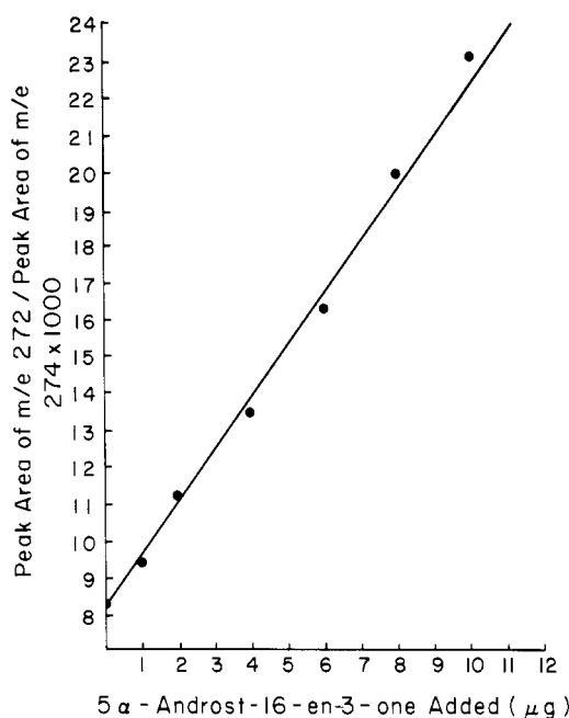
Figure 3. Calibration curve for quantification of 5 \alpha -androst-16-en-3-one.
