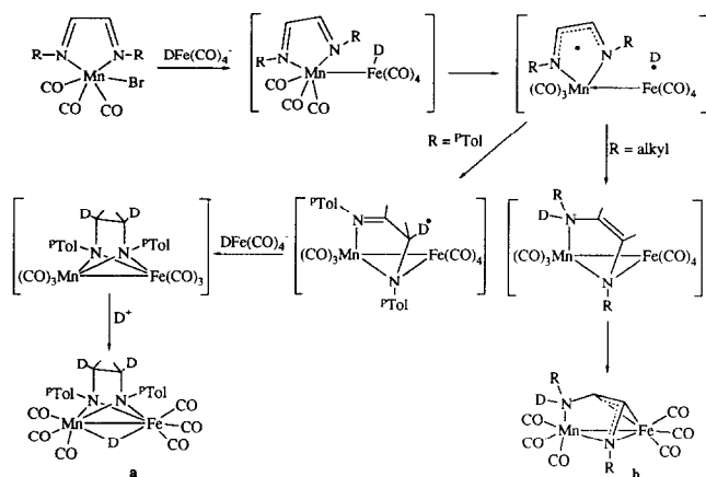
Scheme 1. Proposed mechanism for the formation of (\mu\text{-D})\text{FeMn}(\text{CO})_6(\text{}^p\text{Tol-N-C}(\text{H})(\text{D})\text{C}(\text{H})(\text{D})\text{-N-}^p\text{Tol}) (a) and \text{FeMn}(\text{CO})_6[\text{RNC}(\text{H})\text{C}(\text{H})\text{N}(\text{D})(\text{R})] (b) [7, 8].
