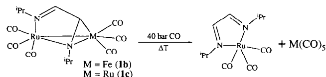
Scheme 5. Reaction of \text{MRu}(\text{CO})_6(\text{}^i\text{Pr-DAB}) ( \text{M} = \text{Fe} ( 1b ); \text{Ru} ( 1c )) with carbon monoxide at high pressure and elevated temperatures.
