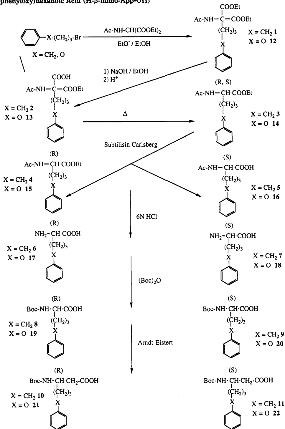
Scheme I. Synthesis of ( R )- and ( S )-3-Amino-7-phenylheptanoic Acid ( H - \beta -homo-Aph-OH) and of ( R )- and ( S )-3-Amino-6-(phenyloxy)hexanoic Acid ( H - \beta -homo-App-OH)
