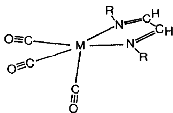
Fig. 1. Molecular structure of the complexes M(\text{CO})_3(\text{R-DAB}) (I: M = \text{Fe} , R = i\text{-Pr}_2\text{Ph} ; III: M = \text{Ru} , R = i\text{-Pr}_2\text{CH} ).
