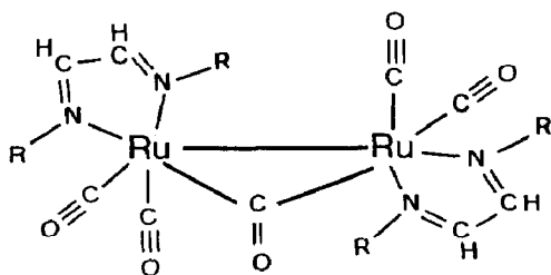
Fig. 8. Proposed structure of \text{Ru}_2(\text{CO})_5(\text{i-Pr}_2\text{CH-DAB})_2 .
