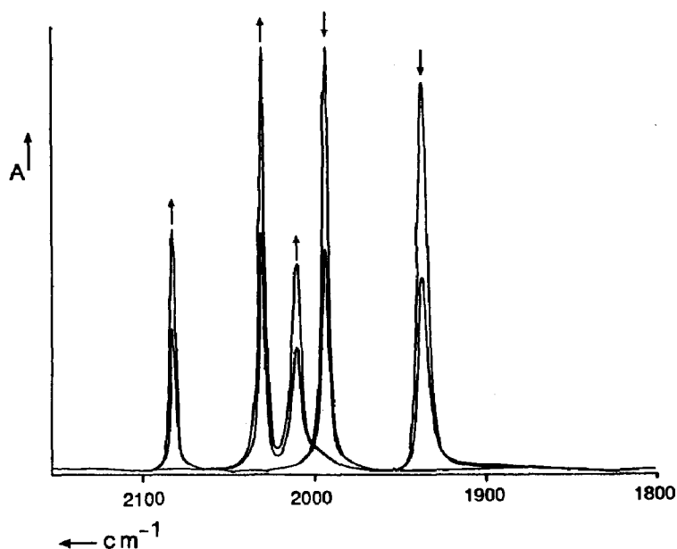
Fig. 4. IR spectral changes (CO-stretching region) accompanying the photochemical conversion of complex IIb into \text{Fe(CO)}_3(\eta^4\text{-i-Pr}_2\text{Ph-DAB}) (n-pentane, 200 K).
