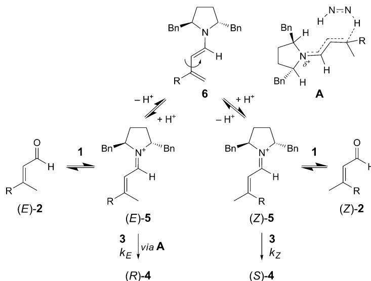
Scheme. Proposed Mechanism of the Organocatalytic Asymmetric Transfer Hydrogenation
