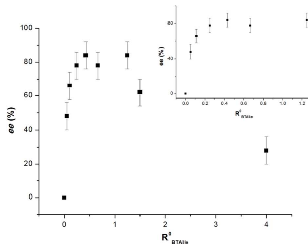
Figure 1. Enantioselectivity of the hydrogenation reaction as a function of R^\circ_{\text{BTAlle}} . R^\circ_{\text{BTAlle}}=n^\circ\text{BTA Ile}/n^\circ\text{BTA}^{\text{PPh}_2} . Inset: zoom on the region for values of R^\circ_{\text{BTAlle}} < 1.5 .
