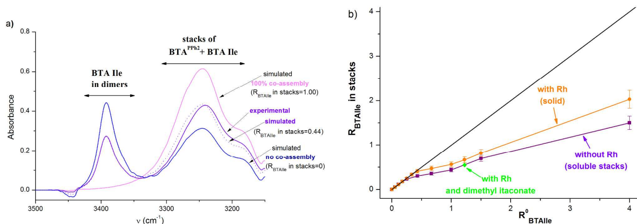
Figure 2. Quantification of the amount of BTA Ile present in the co-assemblies. Left: FT-IR spectrum (zoom on the NH region) of the mixture of BTA PPh 2 and BTA Ile ( R_{\text{BTAIle}}^0=1.00 , [\text{BTA}^{\text{PPh}_2}]^0=8.0 mM) in cyclohexane. Simulated spectra for the extreme cases for which all or no BTA Ile is present in the co-assemblies. R_{\text{BTAIle}} in stacks (here 0.44) is deduced from the amount of BTA Ile in dimers. Right: R_{\text{BTAIle}} in stacks as a function of R_{\text{BTAIle}}^0 (with or without Rh coordinated to BTA PPh 2 ). For the co-assemblies in presence of Rh, the amount of BTA Ile in the insoluble stacks is deduced from the amount of BTA Ile that remains as dimers in the cyclohexane phase. The black line ( y=x ) helps to visualize mixtures for which BTA Ile is fully incorporated into stacks. R_{\text{BTAIle}} in stacks = n_{\text{BTA Ile in stacks}}/n_{\text{BTA}^{\text{PPh}_2}} .
