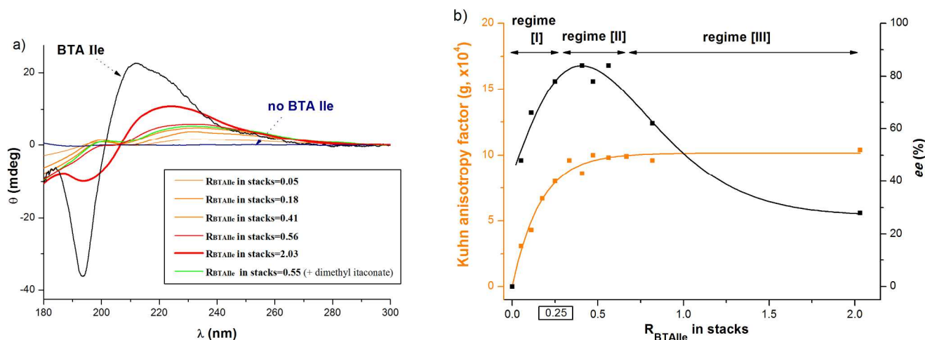
Figure 3. a) CD spectra of the co-assemblies formed between the rhodium complex of ^H\text{BTA}^{\text{PPh}_2} (8 \mu\text{mol} in ^H\text{BTA}^{\text{PPh}_2} for all mixtures) and BTA Ile . For the CD spectra of all the mixtures see Figure S.9. b) Plots of the anisotropy factor ( g ) of co-assemblies and of the enantioselectivity of the hydrogenation reaction as a function of R_{\text{BTAIle}} in stacks. The lines are drawn to guide the eye. g values measured at \lambda=249.0 nm.
