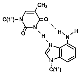
Possible Hoogsteen base pair of c^1c^3A_d and dT
