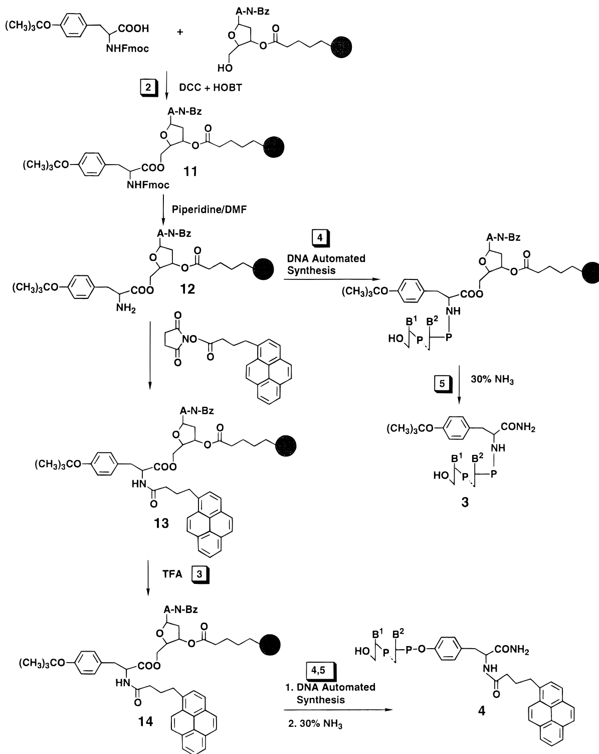
Figure 3. Schematic description of the step by step synthesis of the oligonucleotide conjugates 3 and 4 . The solid support may be both functionalized Teflon and TentaGel (cf. Experimental Section). The conjugate 5 accompanied the conjugate 4 (cf. Experimental Section and Discussion). The numbers in squares indicate the steps 1–5 (Experimental Section).
