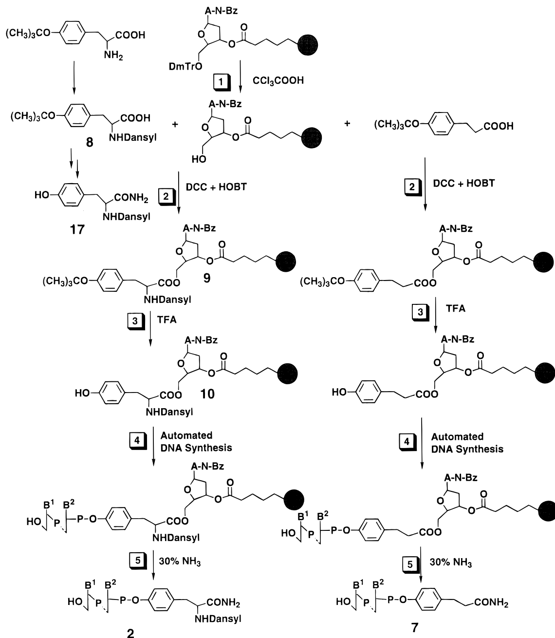
Figure 2. Schematic description of the step by step synthesis of the oligonucleotide conjugates 2 and 7. The solid support may be either functionalized Teflon or TentaGel (cf. Experimental Section). The numbers in squares indicate the steps 1–5 (Experimental Section).
