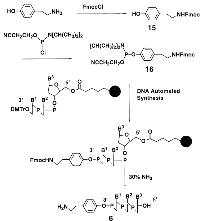
Figure 4. Schematic description of the synthesis of the oligonucleotide conjugate 6 .
