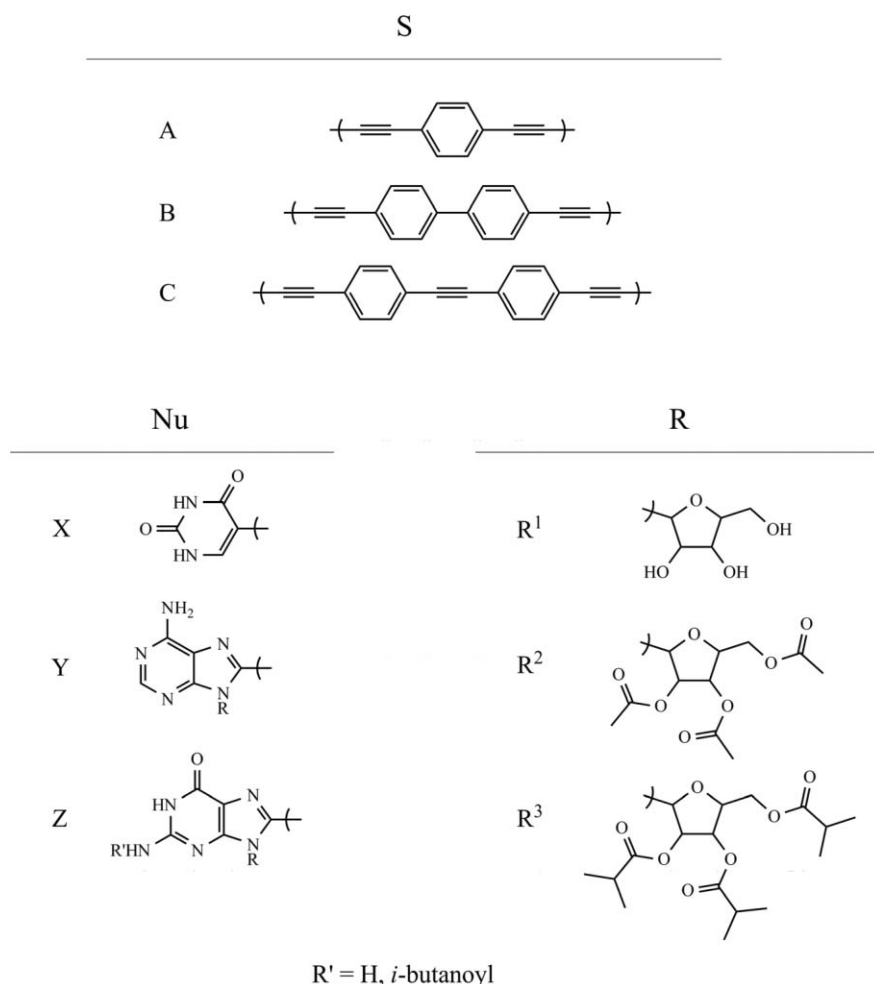
Fig. 4 Linear spacer (A–C), nucleobase and nucleobase derivative (X–Z) constructional components relating to the compound structures of 2–8 (Table 1).
