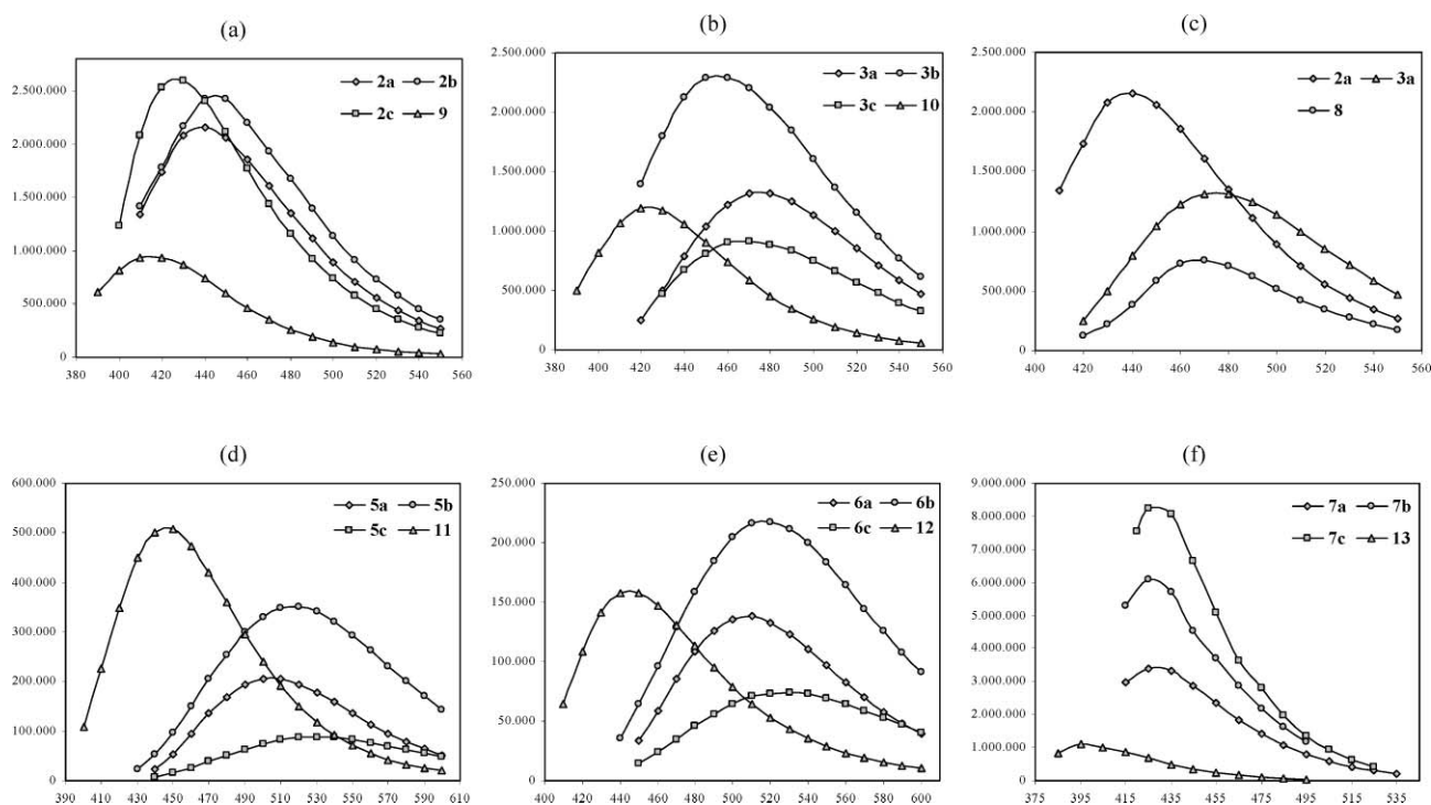
Fig. 12 Fluorescence spectra (0.1 mM solutions of 2 , 3 , 5 , 6 , 8 – 12 in DMSO and 7 , 13 in \text{CHCl}_3 ); intensity (ordinate) against wavelength in nm (abscissa). The individual diagrams relate to derivatives of (a) uracil, (b) adenosine, (c) uracil and adenosine, (d) guanosine, (e) acetyl-protected guanosine, and (f) i -butanoyl-protected guanosine.
