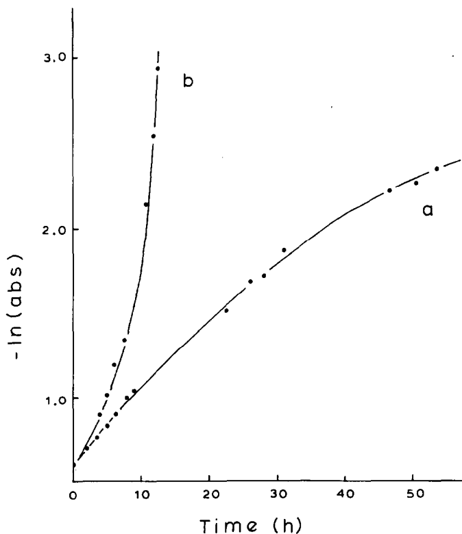
Fig. 2. Plots of -\ln(\text{absorbance}) for \text{HOs}_3(\mu\text{-COMe})(\text{CO})_{10} vs. time for hydrogenation at 90°C (a) in the autoclave at 50 atm and (b) with hydrogen bubbled through the solution.
