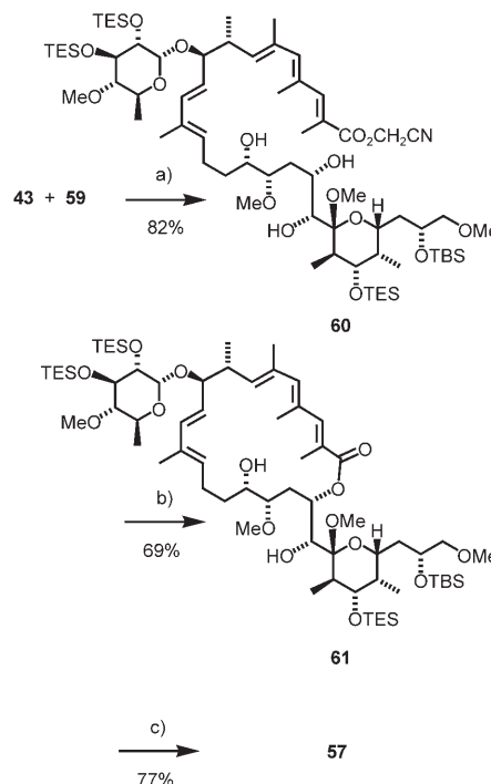
Scheme 11. a) Cu I -thiophene carboxylate, N -methylpyrrolidinone, 0 °C; b) i) LiOH, THF/MeOH, 20 °C; ii) 2,4,6-trichlorobenzoyl chloride, Et 3 N, THF, 6 h; DMAP, toluene; c) H 2 SiF 6 25% in H 2 O, CH 3 CN, -40 → -10 °C.
