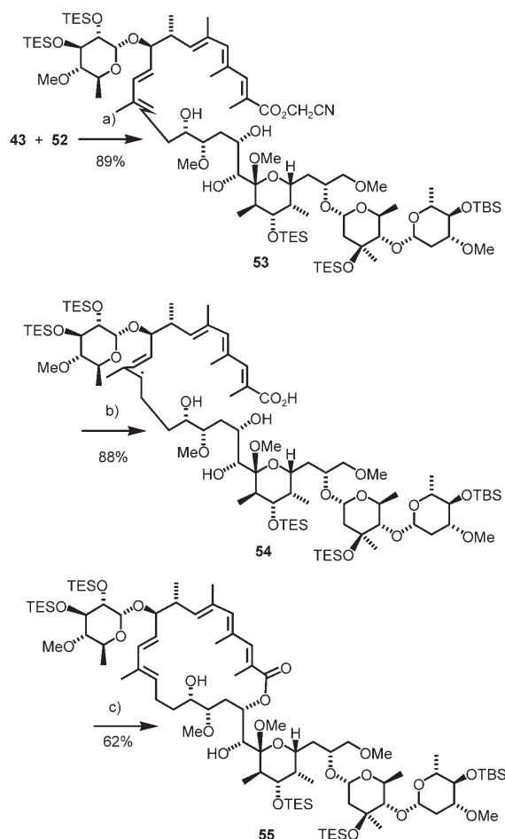
Scheme 8. a) \text{Cu}^{\text{I}} -thiophene carboxylate, N -methylpyrrolidinone, 0^\circ\text{C} ; b) \text{LiOH} , THF/MeOH, 20^\circ\text{C} ; c) 2,4,6-trichlorobenzoyl chloride, \text{Et}_3\text{N} , THF, 6 h; DMAP, toluene.
