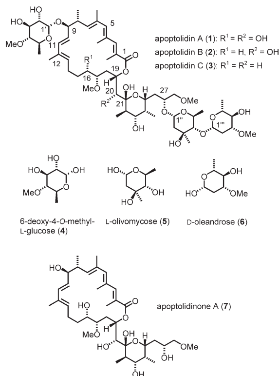
Figure 1. Structures of apoptolidin A, B, C ( 1 , 2 , 3 ), 6-deoxy-4- O -methyl-L-glucose ( 4 ), L-olivomycose ( 5 ), D-oleandrose ( 6 ) and apoptolidinone A ( 7 ).
