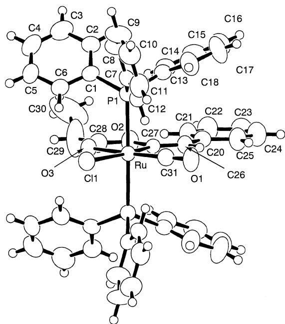
Fig. 1. The molecular structure of 2a with the atom-numbering scheme. Dichloromethane molecules are omitted. The atom numbers in an asymmetric unit are indicated.
