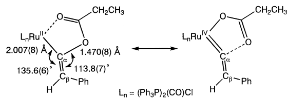
1-acyloxyethenyl chelate ( A )
