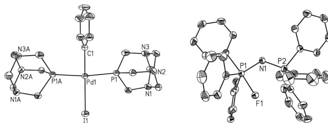
Figure 1. ORTEP drawings of 8 (left) and PPNF (right) with thermal ellipsoids drawn to the 50% probability level and all H atoms omitted for clarity.
