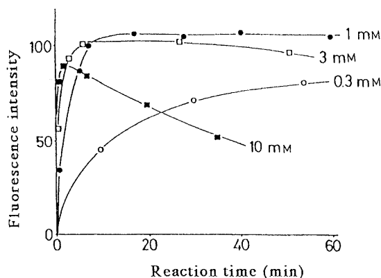
Fig. 2. Time-Courses of Fluorescence Reactions of Various Concentrations of NaIO 4
