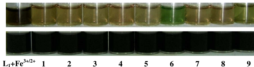
Figure 2. Competitive ion titration of \{\text{L}_1 + \text{Fe}^{3+}\} (bottom row) or \{\text{L}_1 + \text{Fe}^{2+}\} (top row) with different metal ions in methanol: \text{Mg}^{2+} , \text{Ca}^{2+} , \text{Mn}^{2+} , \text{Co}^{2+} , \text{Ni}^{2+} , \text{Cu}^{2+} , \text{Zn}^{2+} , \text{Cd}^{2+} and \text{Hg}^{2+} are present in vials 1–9, respectively.
