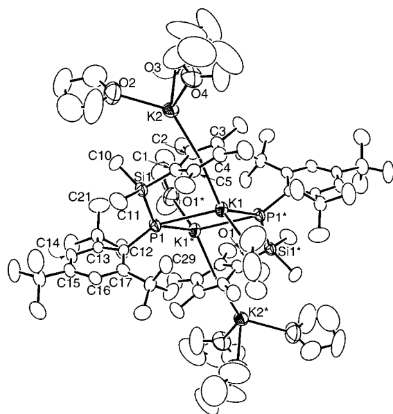
Figure 2. ORTEP drawing of 2 with 30% thermal ellipsoids. Selected bond lengths (Å) and angles (deg): K1–C1, 2.953(8); K1–C2, 3.016(9); K1–C3, 3.114(8); K1–C4, 3.126(8); K1–C5, 3.037(7); K2–C1, 2.959(7); K2–C2, 2.979(7); K2–C3, 3.034(8); K2–C4, 3.02(1); K2–C5, 2.944(8); K1–P1, 3.324(4); K1–P1*, 3.432(2); K1–O1, 2.714(8); K2–O2, 2.72(1); K2–O3, 2.72(1); K2–O4, 2.728(9); P1–Si1, 2.232(3); P1–C12, 1.895(8); Cp'(centroid)–K1–P1, 86.7; Cp'(centroid)–K1–1*, 126.7; Cp'(centroid)–K1–1, 115.3; P1–K1–P1*, 106.53(7); K1–P1–K1*, 73.47(7); K1–Cp'(centroid)–K2, 172.9; O2–K2–Cp'(centroid), 135.0; O3–K2–Cp'(centroid), 117.6; O4–K2–Cp'(centroid), 121.2; O2–K2–O3, 85.3(4); O2–K2–O4, 96.8(4); O3–K2–O4, 86.6(4); K1–P1–C12, 144.8(3); K1–P1–Si1, 85.8(1); Si1–P1–C12, 99.3(2); C10...C21, 3.48; C11...C29, 3.62; C10...C12, 4.15; C11...C12, 3.44; C10–Si1–P1–C12, –84.4(5); C11–Si1–P1–C12, 30.3(5).
