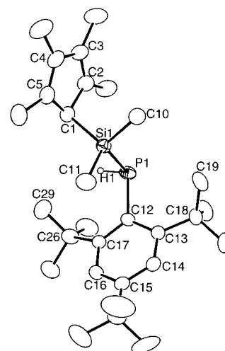
Figure 1. ORTEP drawing of 1 with 30% thermal ellipsoids. Selected bond lengths ( \text{\AA} ) and angles ( ^\circ ): P1–H1, 1.24(6); P1–Si1, 2.310(2); P1–C12, 1.856(4); H1–P1–C12, 102(2); H1–P1–Si1, 96(3); Si1–P1–C12, 100.5(1); P1–Si1–C1, 107.3(1); C1...C29, 3.84; C10...C19, 3.46; C11...C12, 3.26; C10...C12, 4.46; C11–Si1–P1–C12, -9.8(2) ; C10–Si1–P1–C12, 110.8(2) .
