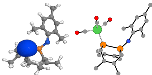
Figure 7. NBO analysis of 1 -NMe 3 shows a well-defined phosphorus lone pair (left, in blue) which can be used for metal binding such as in (OC) 3 Ni(( 1 -NMe 3 )- \kappa^1 P) (right, DFT-optimized structure).
