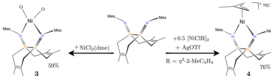
Scheme 5. Syntheses of Nickel(II) Complexes (nppn)NiCl 2 and [(nppn)Ni( \eta^3 -2-C 3 H 4 Me)][OTf]
