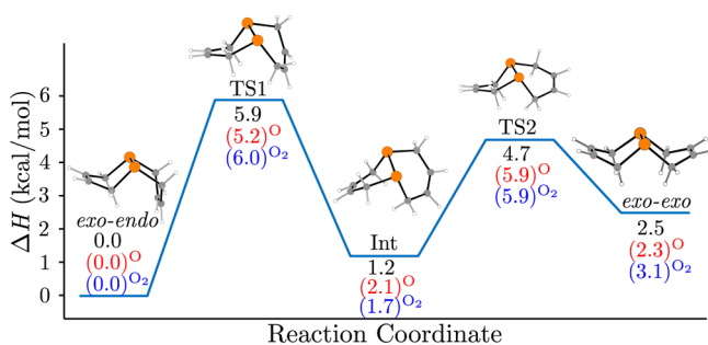
Figure 4. Relative enthalpies for the interconversion of diphosphane 1' (numbers in black) between the endo-exo and the exo-exo conformers (eq 3). Very similar values were observed for the conversions of the monoxide 1'-O (in red) and dioxide 1'-O 2 (in blue) conformers.
