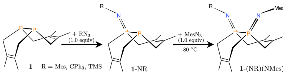
Scheme 3. Synthesis of Mono- and Diiminodiphosphoranes 1 -NR and 1 -(NR)(NMe s )
