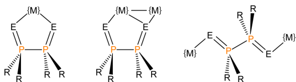
Chart 1. Metal-Binding Modes Available to Diphosphorane Ligands with P–P Bonds
