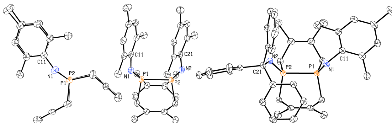
Figure 6. Solid-state structure of the symmetric and the unsymmetric diiminodiphosphoranes 1 -(NMe s ) 2 (left and center) and 1 -(NCPh 3 )(NMe s ) (right) with ellipsoids at the 50% probability level and hydrogen atoms omitted for clarity. Selected interatomic distances [Å] and angles [deg] for 1 -(NMe s ) 2 : P1–P2 2.2398(5), P1–N1 1.5531(13), P2–N2 1.5459(14), N1–P1–P2 120.61(5), N2–P2–P1 120.70(6), C11–N1–P1 140.53(12), C21–N2–P2 140.72(12), N1–P1–P2–N2 5.57(10); and for 1 -(NCPh 3 )(NMe s ): P1–P2 2.2805(7), P1–N1 1.5561(15), P2–N2 1.5504(16), N1–P1–P2 124.25(6), N2–P2–P1 114.39(6), C21–N2–P2 134.51(14), C31–N1–P1 131.48(13), N1–P1–P2–N2 10.95(11).
