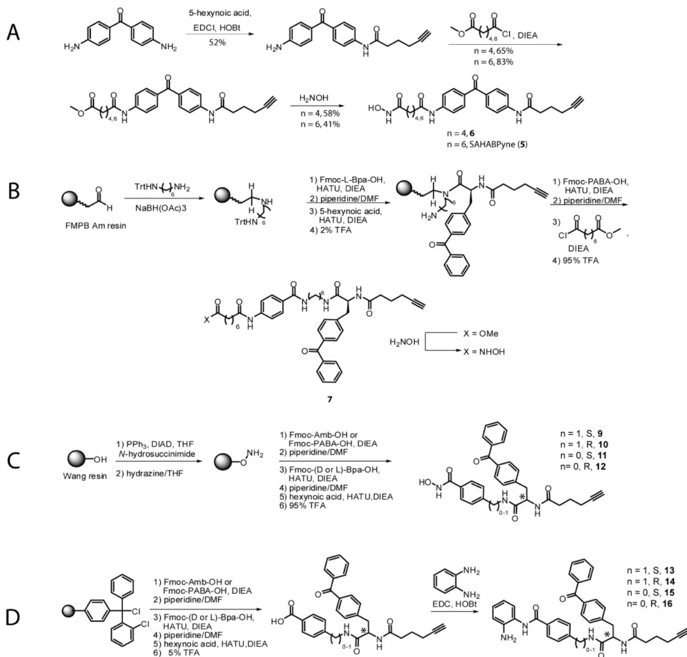
Figure 4. Synthesis of HDAC-directed ABPP probes. (A) Solution-phase synthesis of SAHA-BPyne and shorter linker length analogue 6 . (B) Preparation of 7 , 17 , and 18 were prepared via a similar method, starting with reductive amination of 1-amino-5-hexyne onto FMPB AM resin. (C) Preparation of aryl hydroxamate probes. Probe 19 was prepared by coupling N -Fmoc-Ahx-OH onto O -hydroxylamine resin, followed by deprotection and elaboration via the steps shown. (D) Preparation of benzamide probes.
