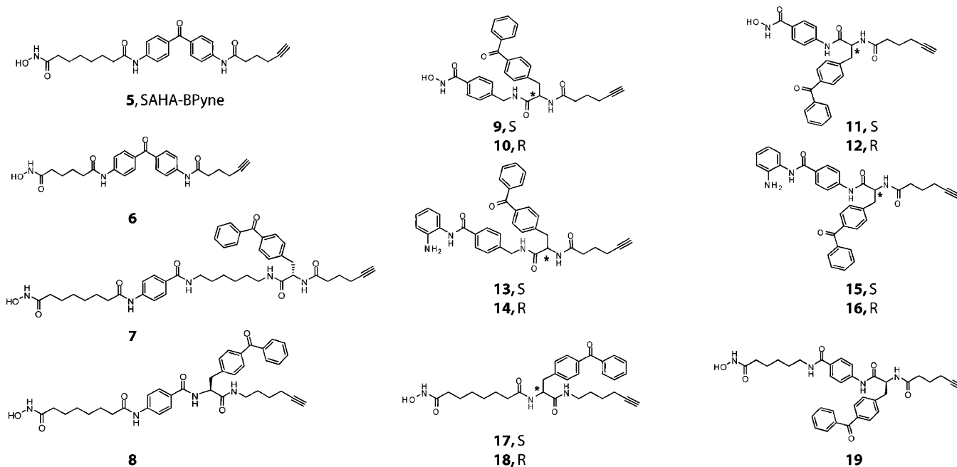
Figure 2. Structures of candidate ABPP probes for HDACs. Stereochemistry of benzophenone amino acid in compounds 9–18 (asterisks) is noted next to the compound numbers.
