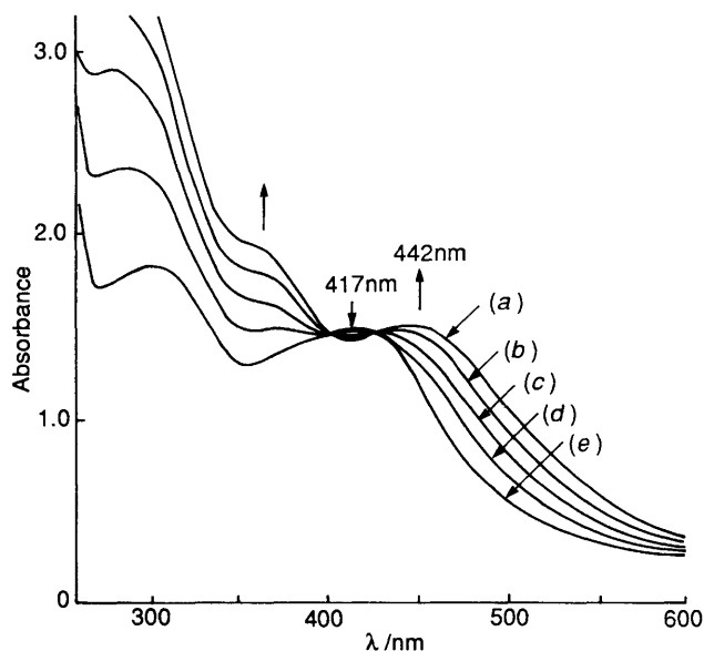
Figure. U.v.-visible titration spectra illustrating ligand exchange (3) + n L 1 → (4) in dmf, where n = ≥ 4 (a), 3 (b), 2 (c), or 1 (d); (e) [Fe 4 S 4 (SBu t ) 4 ] 2- (3) ( n = 0)
