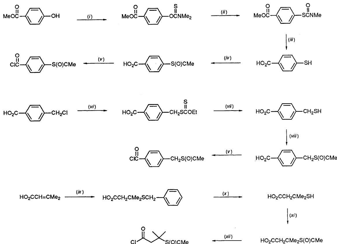
Scheme 2. (i) Me 2 NC(S)Cl, 80%; (ii) 220 °C, 97%; (iii) 10% NaOH-MeOH, 97%; (iv) (MeCO) 2 O, 88%; (v) (COCl) 2 , 80%; (vi) KS 2 COEt, 91%; (vii) H 2 N(CH 2 ) 2 NH 2 , quantitative; (viii) (MeCO) 2 O, 76%; (ix) PhCH 2 SH, 73%; (x) Na-NH 3 , 92%; (xi) (MeCO) 2 O, 69%; (xii) (COCl) 2 , 89%.
