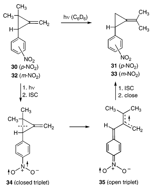
SCHEME 4
