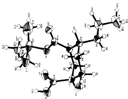
Figure 1: X-ray structure of 8a
