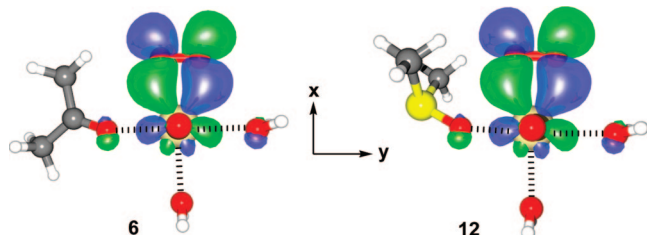
Figure 8. HOMOs ( \beta -spin) for 6 and 12 , showing the strong overlap between the \text{UO}_2^+ 5f_{yz} and \text{O}_2 \pi^*_{xy} orbitals. MOs are rendered at 0.027 (e/\text{\AA}^3)^{1/2} isovalue.
