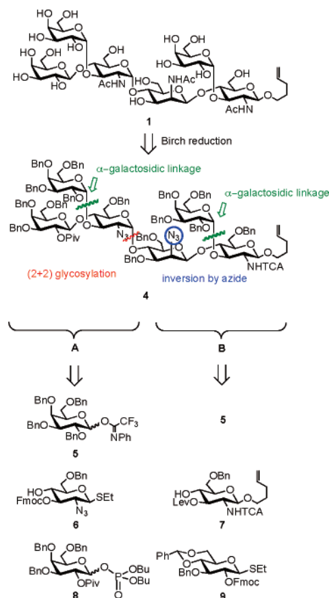
Figure 2. Retrosynthetic analysis.
