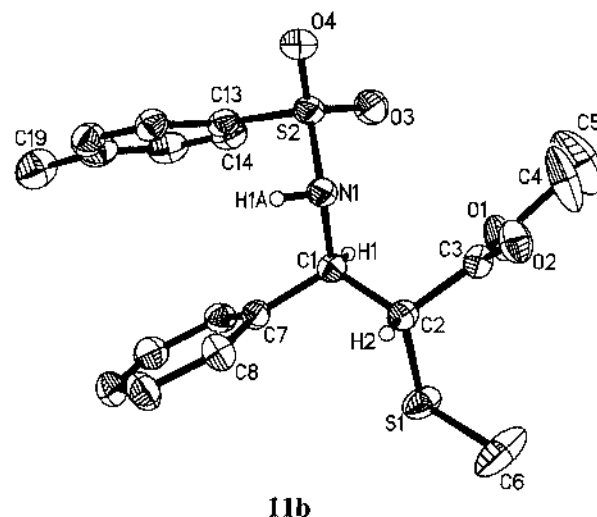
Fig. 2 Solid state molecular structures of 11a and 11b showing one of the four crystallographically independent molecules in each unit cell. Ellipsoids are drawn at the 50% probability level.
