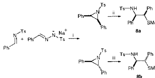
Scheme 6 Reagents and conditions: i, Rh 2 (OAc) 4 (1 mol%), BnEt 3 N + Cl − (10 mol%), 1,4-dioxane, tetrahydrothiophene (20 mol%), 40 °C, 84% (3 : 1, trans : cis ); ii, NaSMe, EtOH, reflux 6 h, 56%; iii, NaSMe, EtOH, reflux 1 h, 97%.
