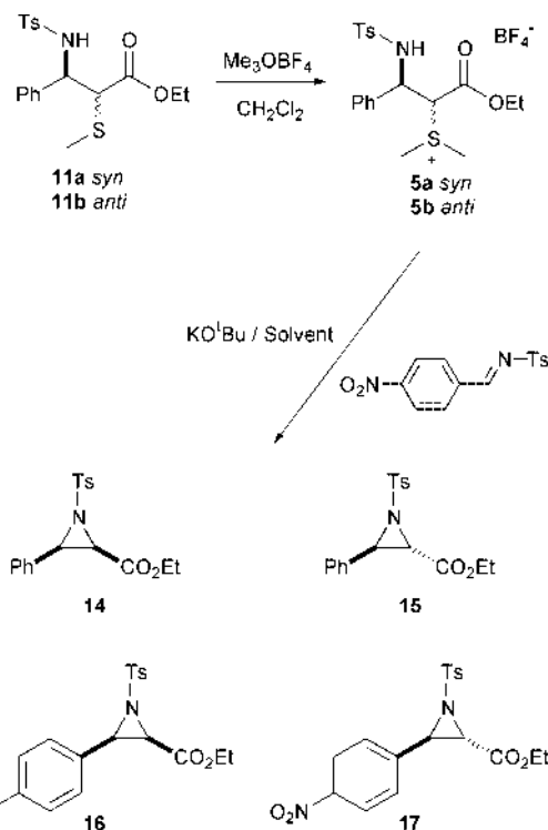
Scheme 12 Cross-over experiments with ester-stabilised sulfur ylide precursors.
