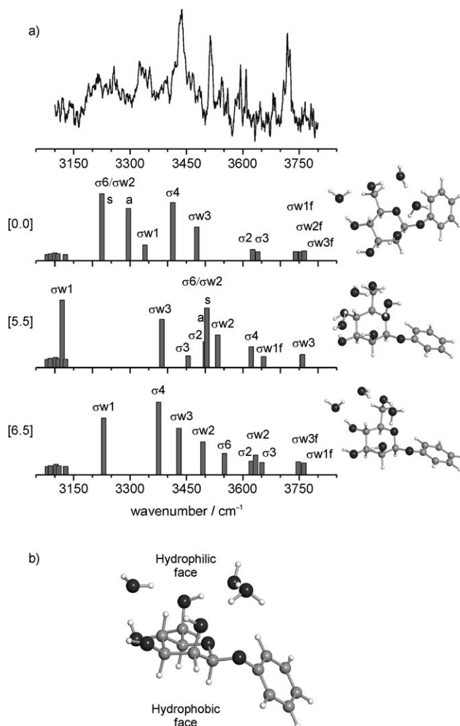
Figure 6. a) Experimental and computed IRID spectra of the trihydrate \beta -D-PhMan \cdot (H 2 O) 3 , cG–g + ·ins(4,6); (6,2;6,2)). Relative energies [kJ mol –1 ] are shown in square brackets. b) A side-on view of the trihydrate, revealing the contrast between the non-hydrated (apolar) and hydrated (polar) faces of the carbohydrate.
