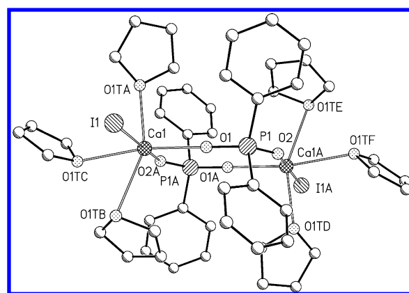
Figure 4. Structural motif of [(\text{thf})_3\text{Ca}(\text{O}_2\text{PPh}_2)\text{I}]_2 ( 3 ) showing the connectivity of the dimer and the formation of an eight-membered (\text{Ca–O–P–O})_2 ring with bridging phosphinate anions. The atoms are drawn with arbitrary radii.
