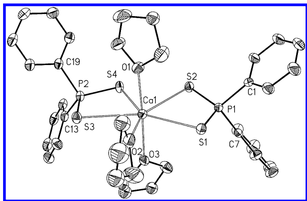
Figure 5. Molecular structure and numbering scheme of [(\text{thf})_3\text{Ca}(\text{S}_2\text{PPh}_2)_2] ( 4 ). The ellipsoids represent a probability of 40%, H atoms are neglected for clarity reasons. Selected bond lengths (pm): Ca1–O1 240.7(2), Ca1–O2 243.5(2), Ca1–O3 237.3(2), Ca1–S1 291.18(10), Ca1–S2 292.17(9), Ca1–S3 294.34(10), Ca1–S4 291.03(10), P1–S1 199.6(1), P1–S2 198.8(1), P2–S3 199.4(1), P2–S4 199.3(1), P1–C1 181.6(3), P1–C7 182.2(3), P2–C13 182.8(3), P2–C19 181.4(3); angles (deg.): S1–Ca1–S2 69.80(2), S1–Ca1–S3 149.17(3), S1–Ca1–S4 140.98(3), S2–Ca1–S3 140.87(3), S2–Ca1–S4 71.47(2), S3–Ca1–S4 69.83(2), O1–Ca1–O2 84.48(10), O1–Ca1–O3 172.15(9), O2–Ca1–O3 87.70(10), O2–Ca1–S1 74.62(7), O2–Ca1–S3 74.59(7).
