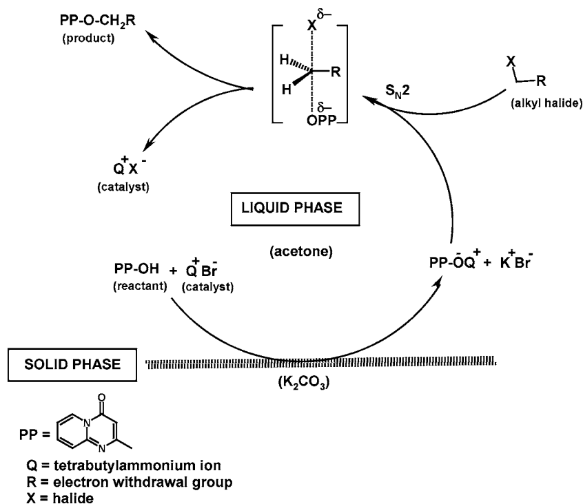
FIGURE 1 PTC alkylation of 2-hydroxypyrido[1,2- a ]pyrimidin-4( H )-one.
