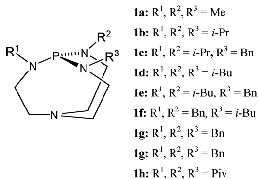
Figure 1. Proazaphosphatranes Ligands.
