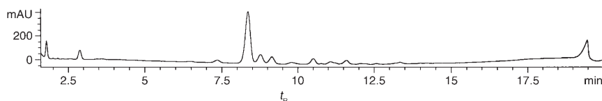
Figure 1. Crude HPLC trace. Product 52 ( t_R = 8.4 min) and its anomers ( t_R = 8.8 and 9.1 min).
