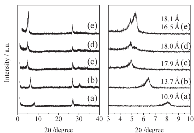
Fig. 2 XRD patterns for (a) dehydrated HNbMoO 6 , (b) hydrated HNbMoO 6 · n H 2 O ( n = 1.23), and (c, e) HNbMoO 6 after immersion in aqueous solution containing (c) glucose, (d) sucrose, or (e) cellobiose.
