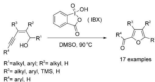
Scheme 1. IBX-mediated formation of 2-acyl furans from cis -enynols.
