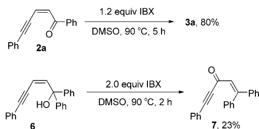
Scheme 4. Reactions of 2a and 6 with IBX.
