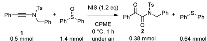
Scheme 1. A byproduct of diphenylsulfane.
