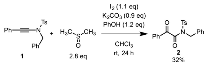
Scheme 3. Oxidation of 1 under Matsumoto's condition.
