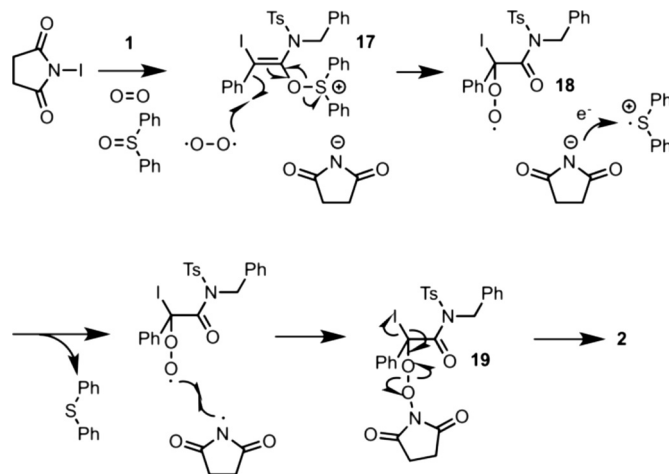
Fig. 1. Plausible reaction path to 2 via 17 , 18 , and 19 .
