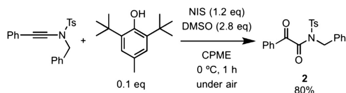
Scheme 2. The oxidation in the presence of 2,6-di- tert -butyl-4-methyl phenol.
