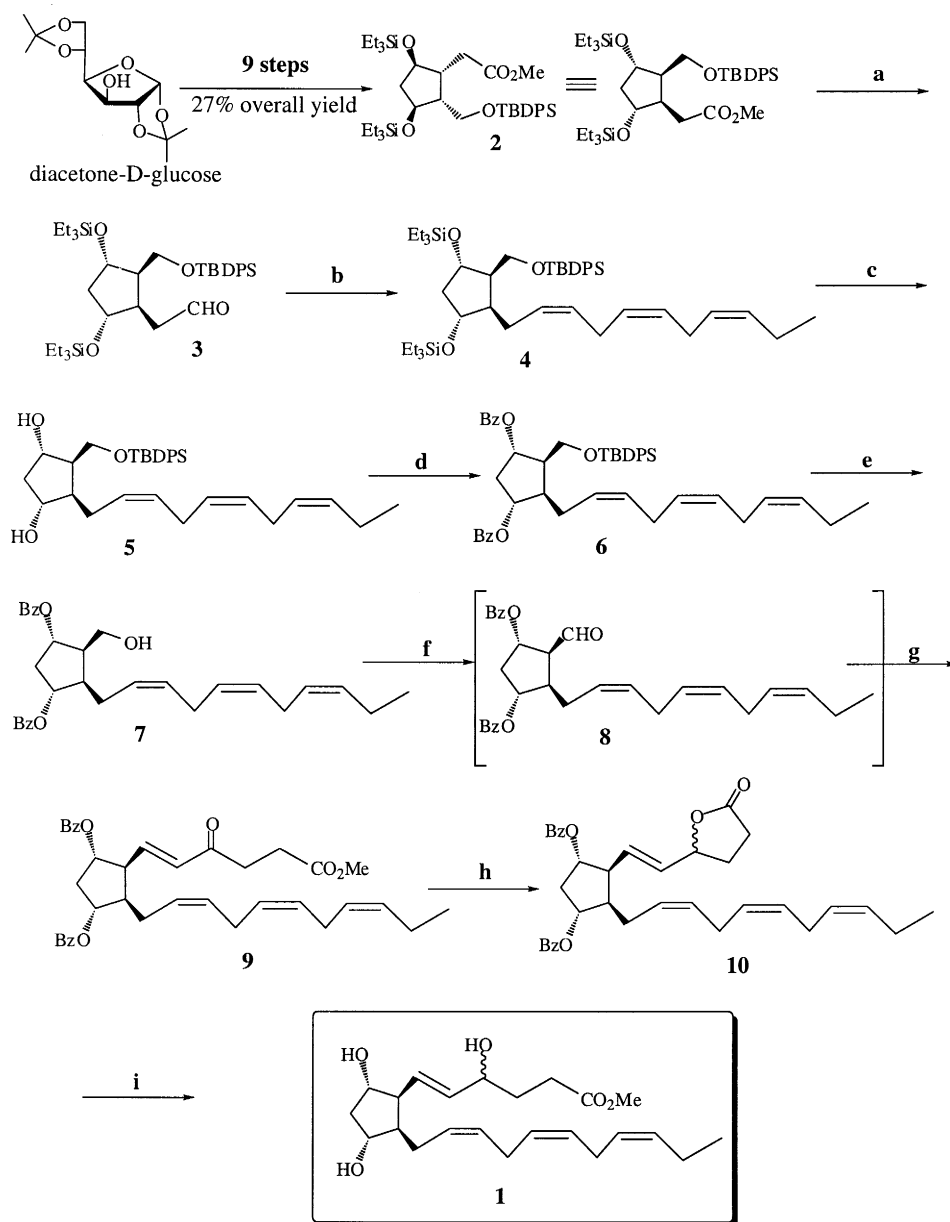
Scheme 2. (a) 1.1 equiv. DIBAL-H (1 M in toluene), toluene, -80^{\circ}\text{C} , 30 min, 93%; (b) 4 equiv. [( Z,Z )-3,6-nonandiene-1-yl] triphenylphosphonium iodide, 3.8 equiv. \text{NaN}(\text{SiMe}_3)_2 , THF, -80^{\circ}\text{C} to 20^{\circ}\text{C} , 2 h, 68%; (c) \text{NH}_4\text{F} , THF–MeOH, 4 h, 92%; (d) 4 equiv. \text{BzCl} , pyridine, 20^{\circ}\text{C} , 1 h, 86%; (e) \text{HCl} 3% in MeOH, 20^{\circ}\text{C} , overnight, 73%; (f) periodinane, \text{CH}_2\text{Cl}_2 , rt, 2 h; (g) 1.2 equiv. diethyl[4-(methoxycarbonyl)-oxobutyl]phosphonate, 1.1 equiv. \text{NaN}(\text{SiMe}_3)_2 , THF, 20^{\circ}\text{C} , 30 min, 64%; (h) 1.1 equiv. L-Selectride®, THF, -78^{\circ}\text{C} , 20 min, 65%; (i) 1N NaOH, THF–MeOH, rt, 1 h, then \text{CH}_2\text{N}_2 63%
