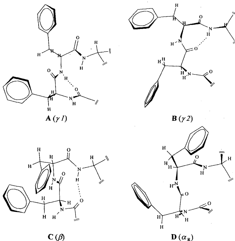
Fig. 1. Possible conformations of the peptide chains: \gamma^1 -loop A between NH (Phe2) and CO (Spa'), \gamma^1 -loop B between NH (Spa) and CO (Phe1), \beta -loop C between NH (Spa) and CO (Spa'), and \alpha -helical conformation D
