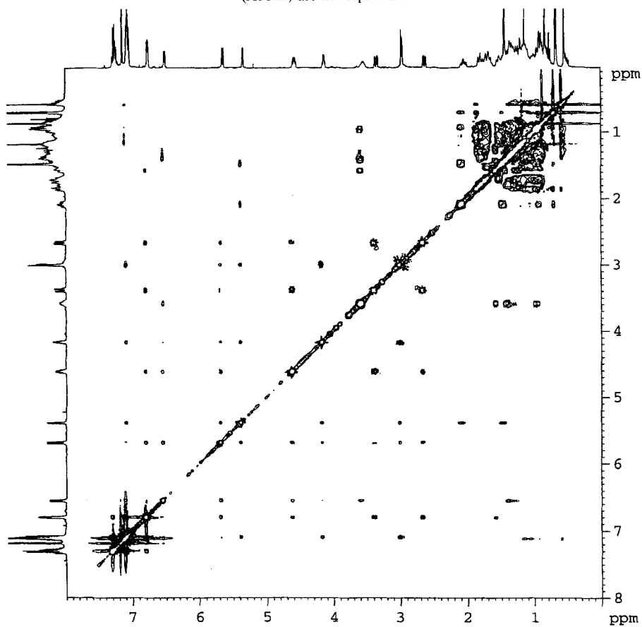
Fig. 3. 2D-ROESY Spectrum of 1a in \text{CDCl}_3 at 30^\circ . Mixing time 250 ms.
