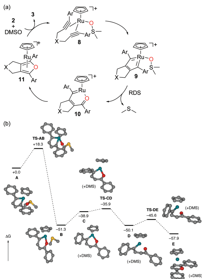
Figure 1. (a) Proposed mechanism. (b) Calculated energy surface with relative Gibbs free energies \Delta G (kcal/mol) at 298 K.
