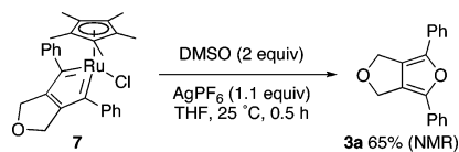
Scheme 5. Reaction of Ruthenacycle 7 with DMSO
