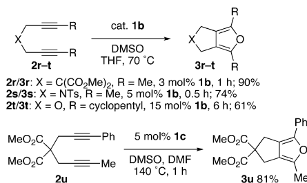
Scheme 3. Synthesis of Furans from Diynes with Alkyl Terminal Groups
