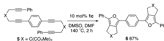
Scheme 4. Double Transfer Oxygenative Cyclization of Tetraynes
