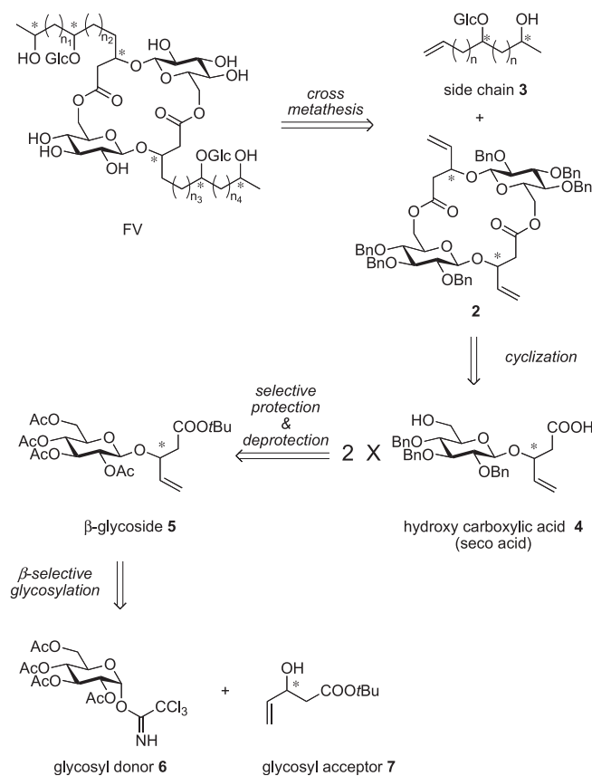
Scheme 2. Retrosynthetic analysis.
