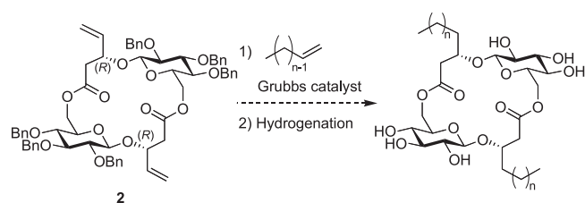
Scheme 1. Late stage of synthetic plan.
