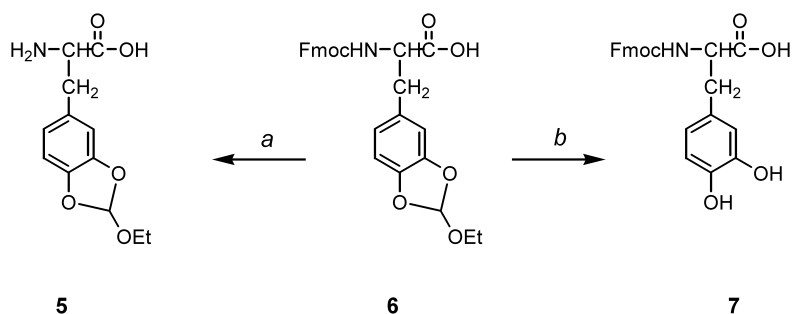
Scheme 2. Reagents and conditions: (a) 25% piperidine/DMF, rt, 60 h; (b) 1 M TMSBr/TFA, thioanisole, m -cresol, EDT, 0°C, 60 min
