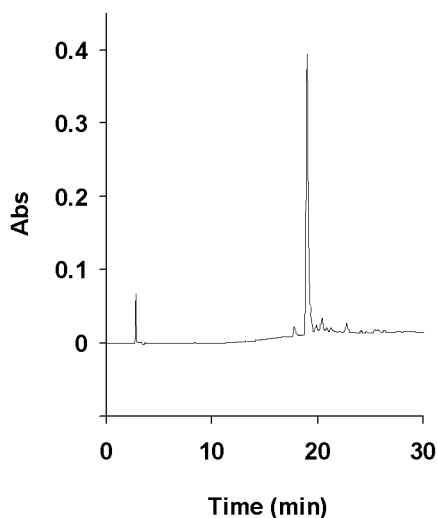
Figure 1. RP-HPLC of the crude decapeptide. HPLC was performed on a Vydac C18 reversed-phase column (250×4.6 mm, 10 μm) with a linear gradient 5–35% CH 3 CN in 0.1% TFA (v/v) over 30 min, flow rate 1.0 ml/min, and UV detection at 215 nm; 2 μl (2.5 mg/ml) of sample was injected
