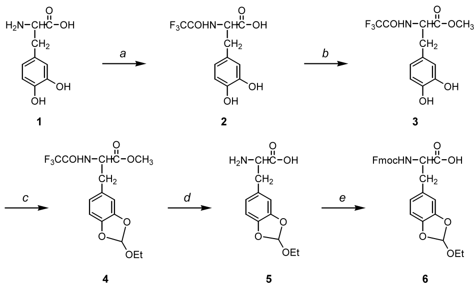
Scheme 1. Reagents and conditions: (a) \text{CF}_3\text{CO}_2\text{Me} , \text{NEt}_3 , MeOH, rt, 6 h, 95%; (b) \text{CH}_3\text{I} , \text{KHCO}_3 , DMF, rt, 4 h, 95%; (c) \text{HC}(\text{OEt})_3 , TsOH, molecular sieves 4A, benzene, reflux, 3 d, 80%; (d) NaOH, THF/ \text{H}_2\text{O} , rt, 16 h; (e) Fmoc-OSu, THF/ \text{H}_2\text{O} , rt, 8 h, 80% (d and e)
