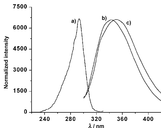
Figure 8. The excitation spectrum of a) GOx, and the fluorescence spectra of b) GOx and c) GOx conjugated on the CdTe QDs.
