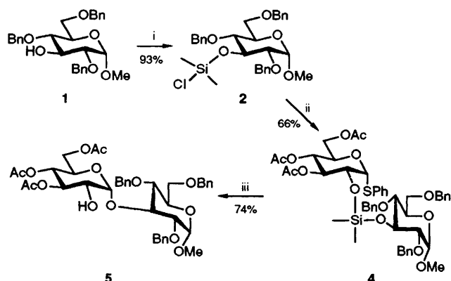
Scheme 1 Reagents and conditions: i, \text{Me}_2\text{SiCl}_2 , \text{Et}_3\text{N} , diethyl ether; ii, 3a , pyridine, THF; iii, NIS, \text{MeNO}_2 , 100 °C, 1 h
