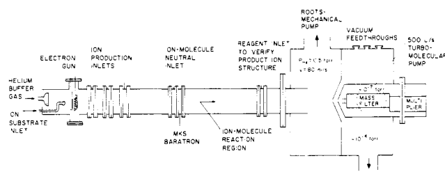
Figure 1. Diagram of the flowing afterglow apparatus.
