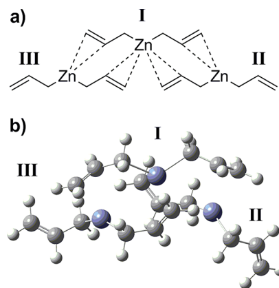
Figure 3. Lewis drawing (a) and calculated structure (b) of the bis( \eta^1 -allyl)zinc trimer optimized at the MP2/aug-cc-pVDZ level of theory.
