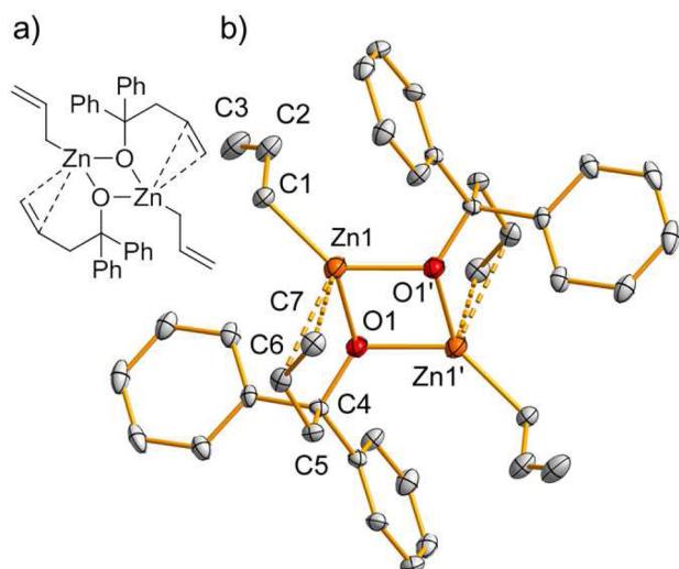
Figure 5. Lewis drawing (a) and molecular structure (b) of the dimer of [\text{Zn}(\eta^1\text{-C}_3\text{H}_5)(\text{OC}(\text{C}_3\text{H}_5)\text{Ph}_2)] ( 3 ). Displacement ellipsoids are shown at the 50% probability level. Hydrogen atoms are omitted for clarity. Selected bond lengths (Å) and angles (deg): Zn1–C1, 1.976(4); Zn1–C6, 2.741(4); Zn1–C7, 2.619(4); Zn1–O1, 1.975(2); C1–C2, 1.485(7); C2–C3, 1.280(8); C4–O1, 1.429(5); C4–C5, 1.544(6); C5–C6, 1.502(6); C6–C7, 1.325(6); C1–Zn1–center(C6–C7), 107.0(1); C1–Zn1–O1, 134.9(1); C1–Zn1–O1', 135.2(1); center(C6–C7)–Zn1–O1, 82.2(7); center(C6–C7)–Zn1–O1', 101.0(8); O1–Zn1–O1', 82.7(1); Zn1–O1–Zn1', 97.3(1); C1–C2–C3, 129.9(5); C5–C6–C7, 124.9(4). Primed atoms are related by symmetry code [-x, -y, -z] .
