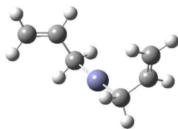
Figure 2. Structure of bis( \eta^1 -allyl)zinc optimized at the MP2/aug-cc-pVDZ level of theory.
