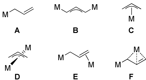
Scheme 1. Coordination Modes of the Allyl Ligand Involving Carbon Metal Interactions of \sigma -Type (A: \eta^1 ; B: \mu_2\text{-}\eta^1\text{:}\eta^1 ( cis and trans Isomer Possible)), \pi -Type (C: \eta^3 ; D: \mu_2\text{-}\eta^3\text{:}\eta^3 ), or \sigma - and Possibly \pi -Type (E: \mu_2\text{-}\eta^1\text{:}\eta^2 ; F: \mu_2\text{-}\eta^1\text{:}\eta^3 )
