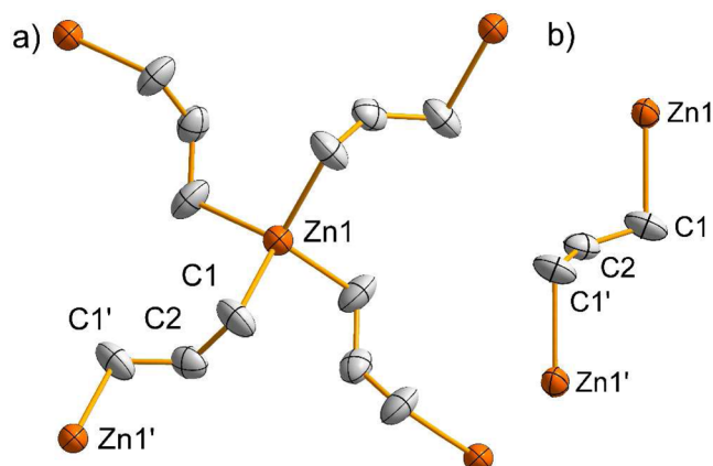
Figure 1. Cut-out of the solid state structure of bis(allyl)zinc ( 1 ): (a) three-dimensional network of 1 ; (b) \text{trans } \mu_2\text{-}\eta^1\text{:}\eta^1 coordination mode of the allyl ligand. Displacement ellipsoids are shown at the 50% probability level. Both symmetrically independent carbon atoms of the ligand occupy general positions; this implies 2-fold disorder for C2. Only one of the two split positions for C2 is shown. Hydrogen atoms are omitted for clarity. Bond lengths (Å) and angles (deg): Zn1–C1, 2.171(2); C1–C2, 1.423(4); C2–C1', 1.333(5); C1–Zn1–C1', 103.86(12); C1–Zn1–C1'', 112.36(8); C1–C2–C1', 130.6(3). Primed atoms are related by symmetry code [\frac{3}{2} - x, \frac{3}{2} - y, \frac{1}{2} - z] .
