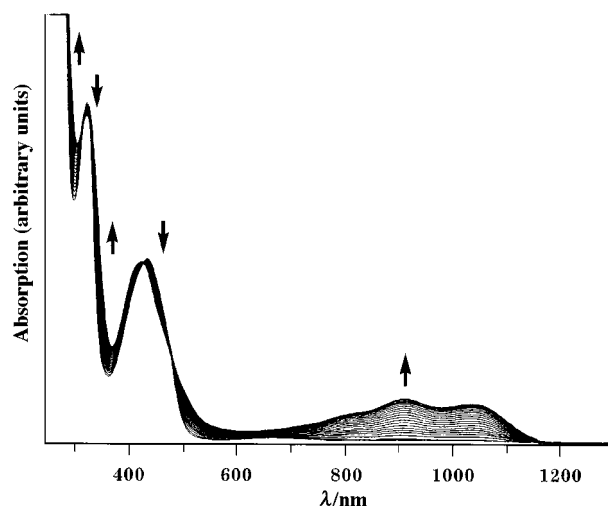
Fig. 6 Oxidation of complex 2 to [2] + by controlled potential electrolysis in CH 2 Cl 2 –0.5 M NBu 4 PF 6 at 243 K.
