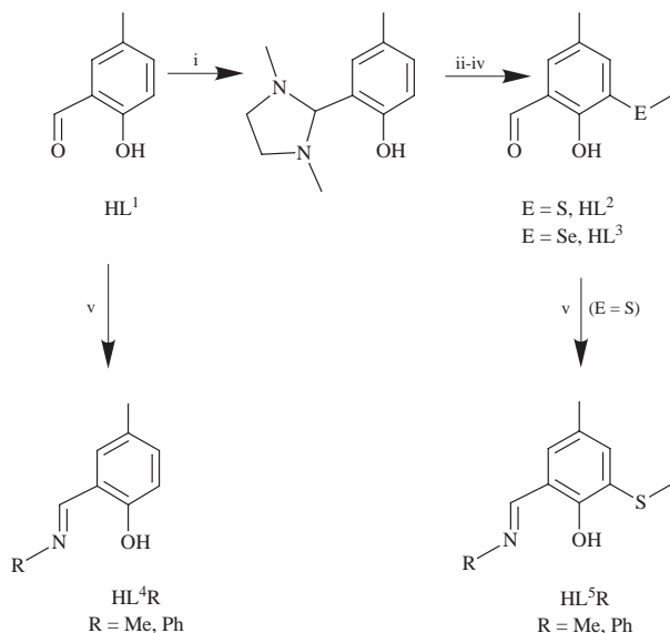
Scheme 1 (i) DMEDA, EtOH, \text{MgSO}_4 , RT, 16 h; (ii) 4 equivalents \text{Bu}^n\text{Li}/\text{TMEDA} , \text{Et}_2\text{O} , -78^\circ\text{C} to RT, 6 h; (iii) \text{MeEEMe} ( \text{E} = \text{S} or \text{Se} ), RT, 16 h; (iv) 2 M \text{HCl} , RT, 10 min; (v) \text{RNH}_2 , \text{MeOH} .
