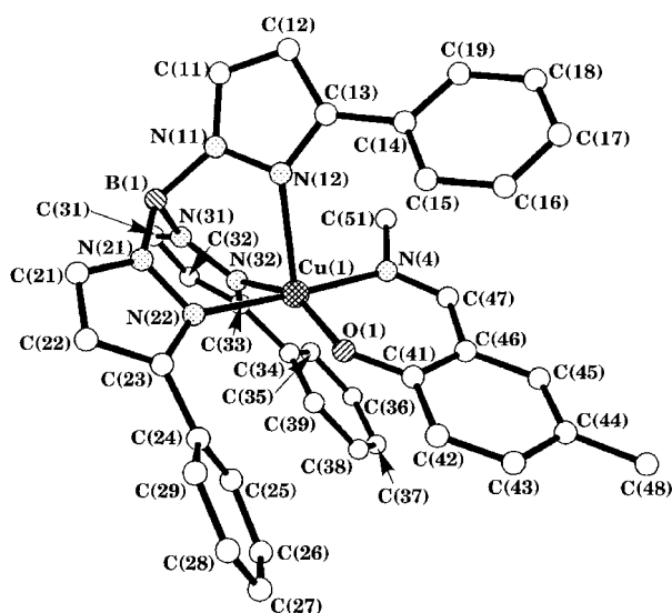
Fig. 3 Structure of the [\text{Cu}(\text{L}^4\text{Me})(\text{Tp}^{\text{Ph}})] complex molecule in the crystal of 4 \cdot \text{CH}_2\text{Cl}_2 . Details as for Fig. 2.
